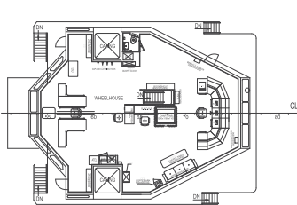
Bridge deck
