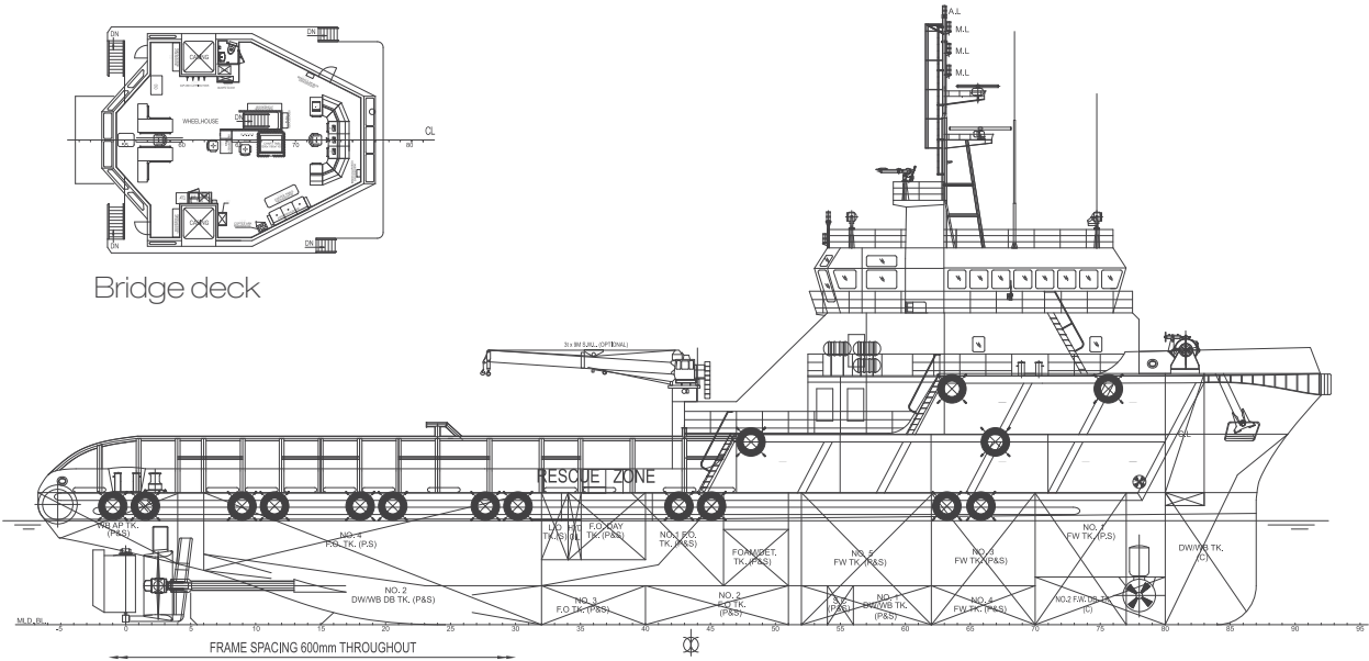
Outboard profile
