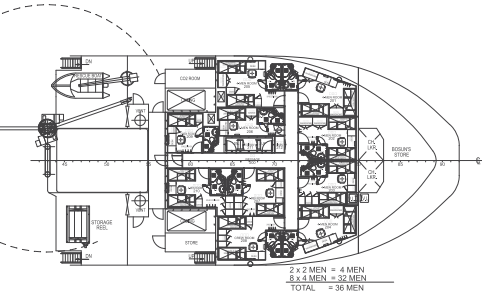
Forecastle deck
