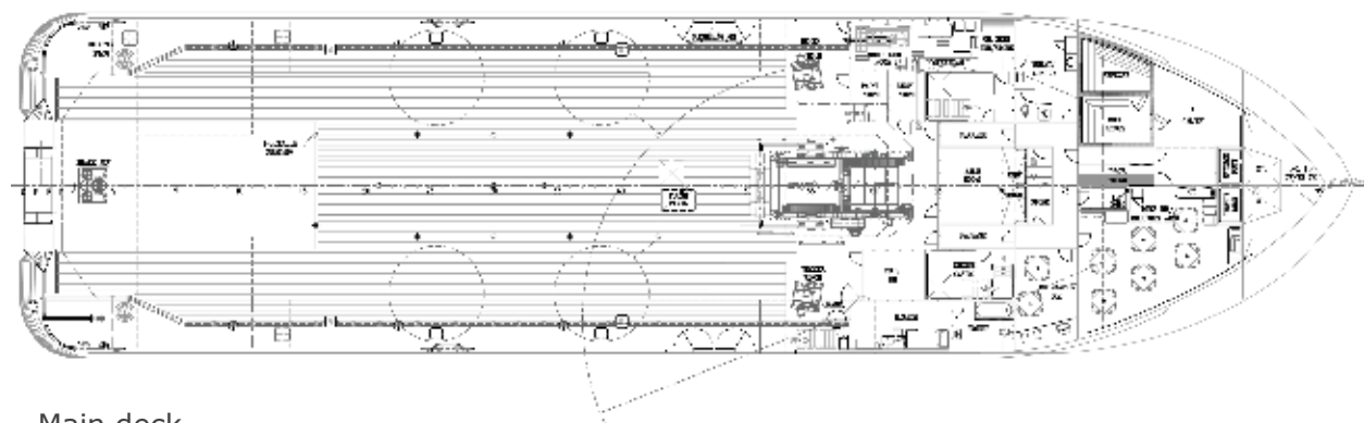
Main deck
