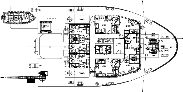
Forecastle deck
