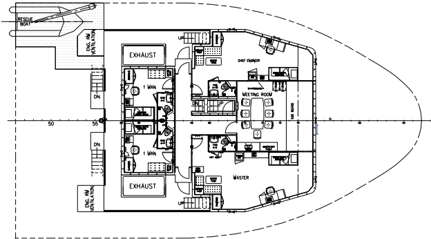
Bridge Deck
