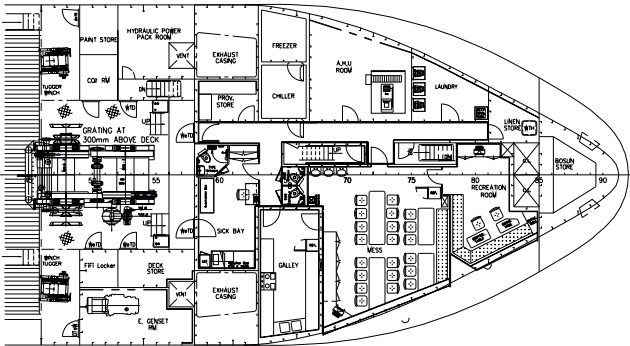
Raised deck
